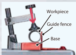
Stand set (option)
